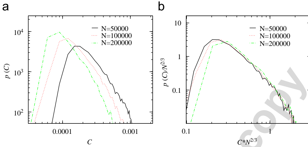
Fig. 5. The dependence of p(C) on the system size N with p = p_c for (a) before scaling and (b) after scaling. Simulations are performed on ER networks with \langle k \rangle = 3 .
