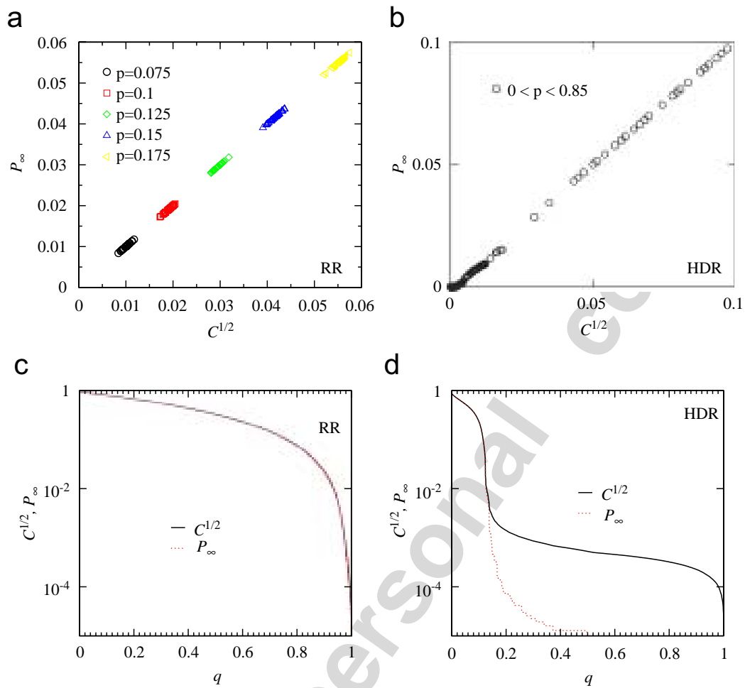
Fig. 7. P_\infty versus C^{1/2} for (a) RR strategy and (b) HDR strategy and plot C^{1/2} , P_\infty versus q for (c) RR strategy and (d) HDR strategy for the Swedish network of workplaces with N = 310136 nodes.
