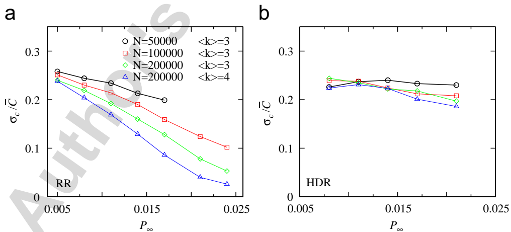
Fig. 4. The dependence of \sigma_C/\bar{C} for (a) RR and (b) HDR on system size N and average degree \langle k \rangle of ER networks.
