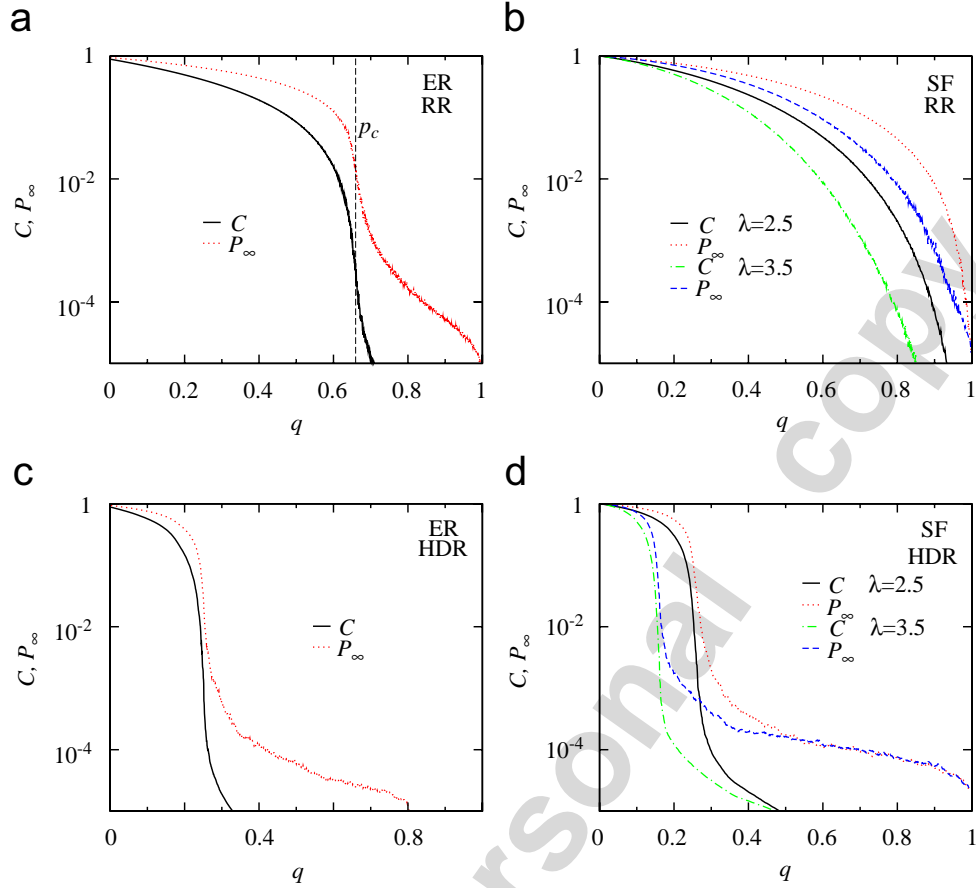
Fig. 1. The behavior of C and P_\infty versus q on ER and SF networks. For ER networks, N = 200\,000 and \langle k \rangle = 3 . For SF networks, N = 80\,000 . The graphs are (a) RR strategy on ER networks, (b) RR strategy on SF networks, (c) HDR strategy on ER networks and (d) HDR strategy on SF networks.
